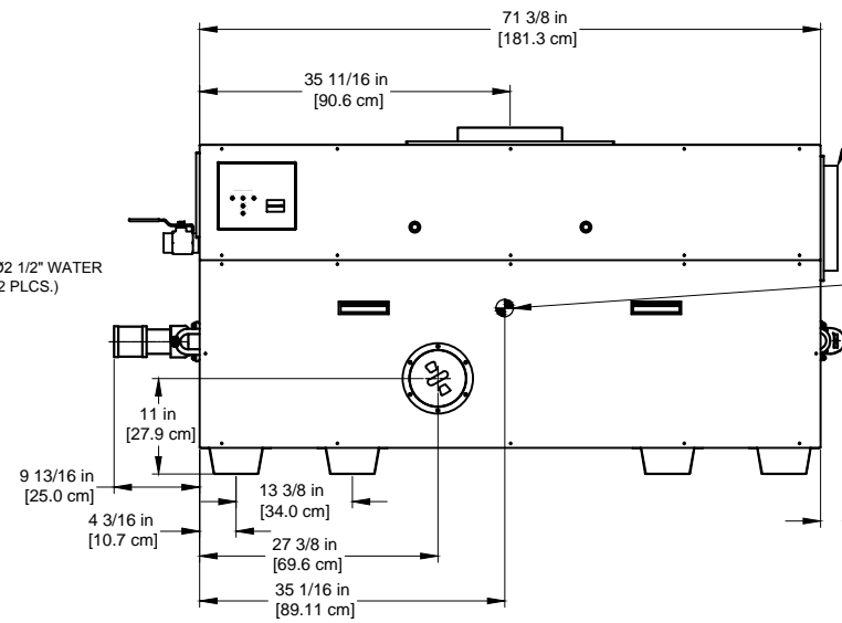
FRONT
