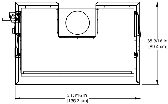
OUTDOOR TOP PANEL
