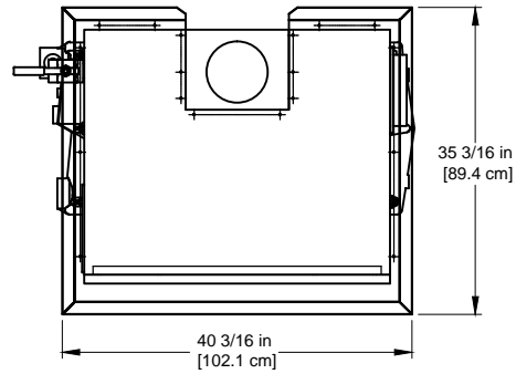
OUTDOOR TOP PANEL
