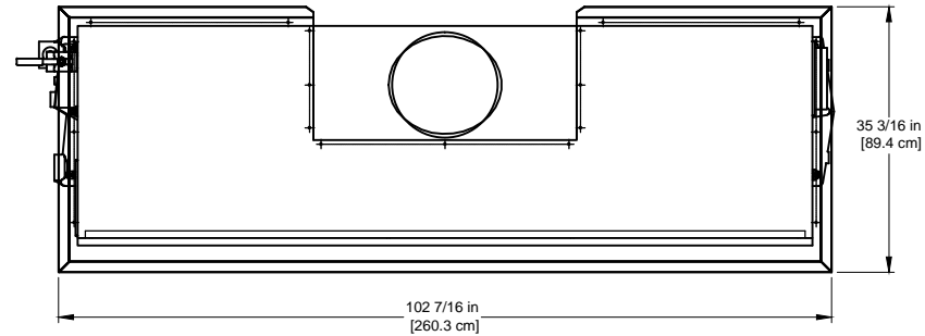
OUTDOOR TOP PANEL
