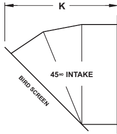
WALL INTAKE HOOD
