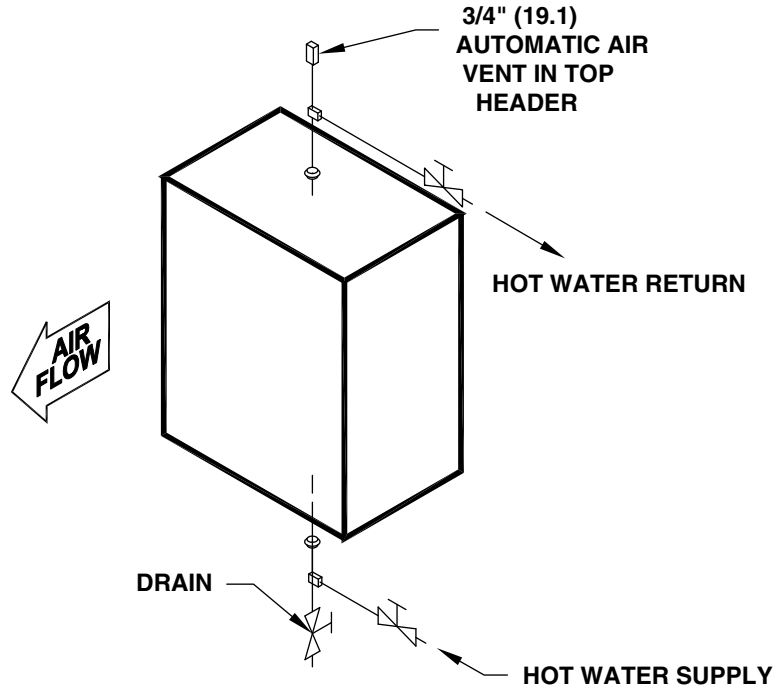
DOUBLE SECTION - 4 ROW COIL
