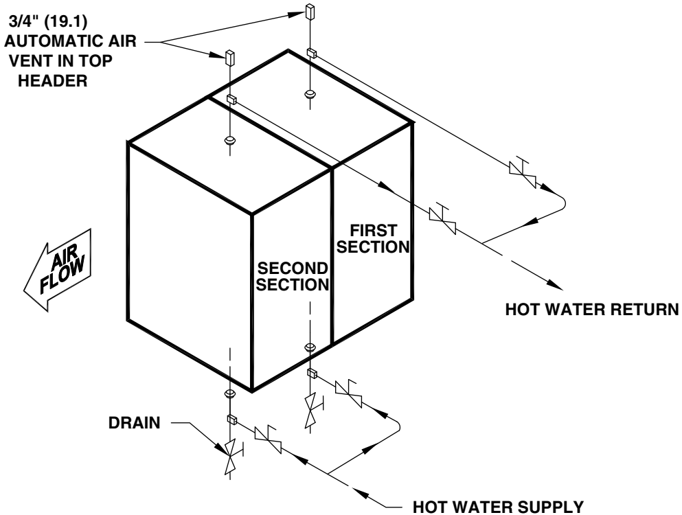
DOUBLE SECTION - 4 ROW COIL
