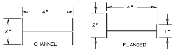
TYPICAL FABRICATED RADIUS CONFIGURATION
