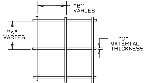
GRID SPACING DETAIL
