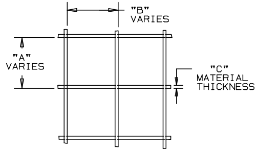
GRID SPACING DETAIL
