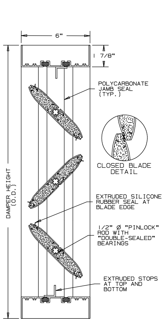
OPPOSED BLADE DAMPER (SHOWN) PARALLEL BLADE DAMPER AVAILABLE
