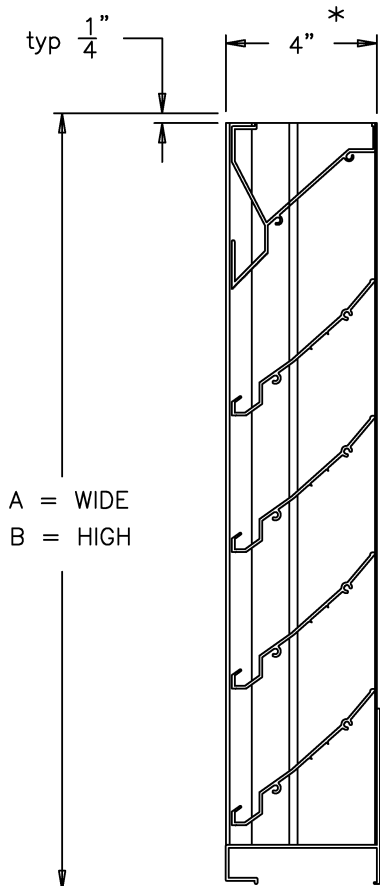
SECTION VIEW
