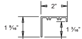
Frame Option 2 Flange Frame 2" or 4" Deep, .080" Thick
