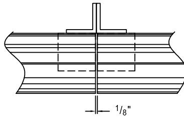
Optional Architectural Vertical Mullion
